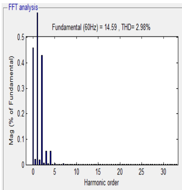
Figure 5. harmonic order A Combination of Shunt Hybrid Power Filter and Thyristor-Controlled Reactor in steady state condition
