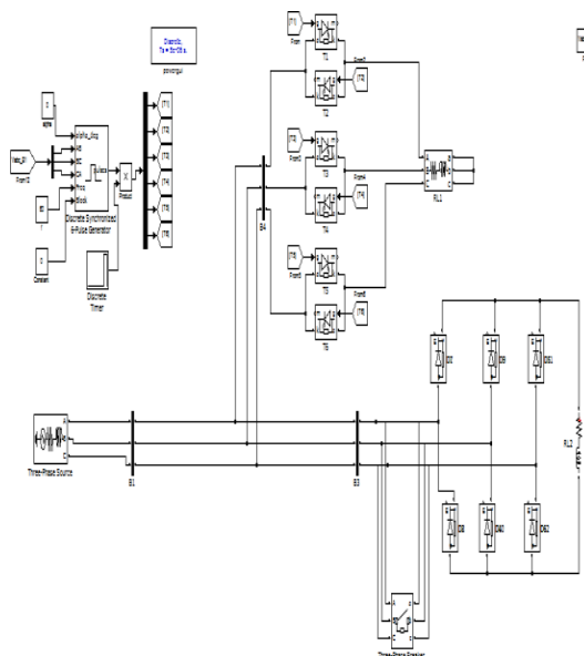
Figure 3. conventional circuit configuration
