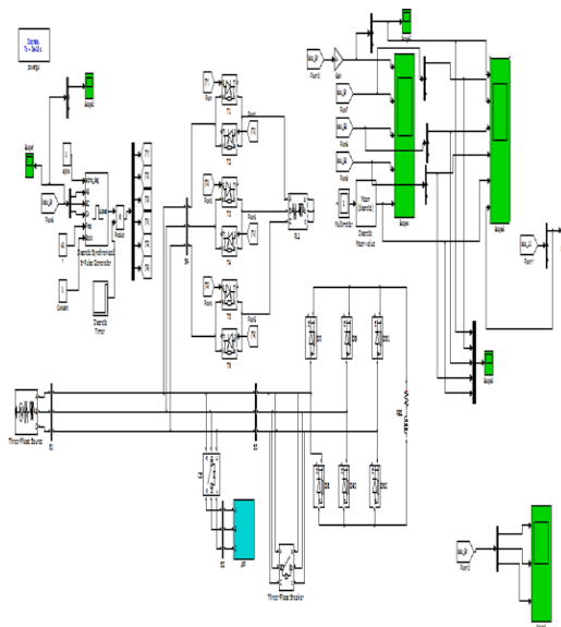
Figure 4. A Combination of Shunt Hybrid Power Filter and Thyristor-Controlled Reactor in steady state condition
