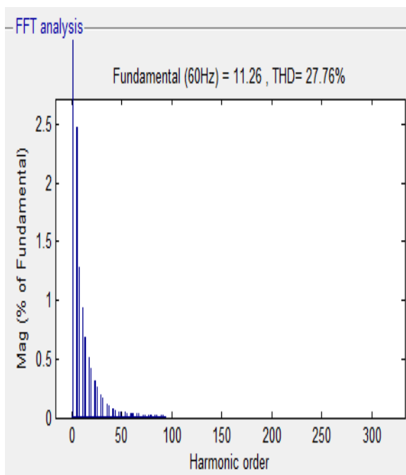
Figure 4. harmonic order for the conventional circuit configuration.
