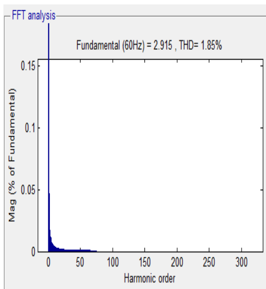
Figure 8. harmonic order A Combination of ShuntHybrid Power Filter and Thyristor-Controlled Reactor in dynamic state condition
