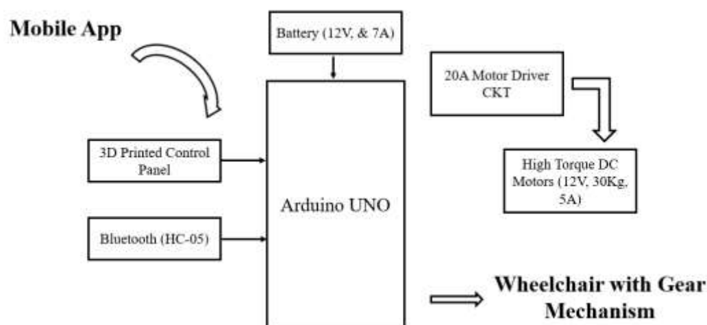
Figure 2: Proposed block diagram of voice controlled real-time wheelchair with gear mechanism.
