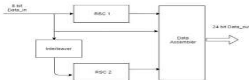
Figure 2. Turbo encoder operation.
