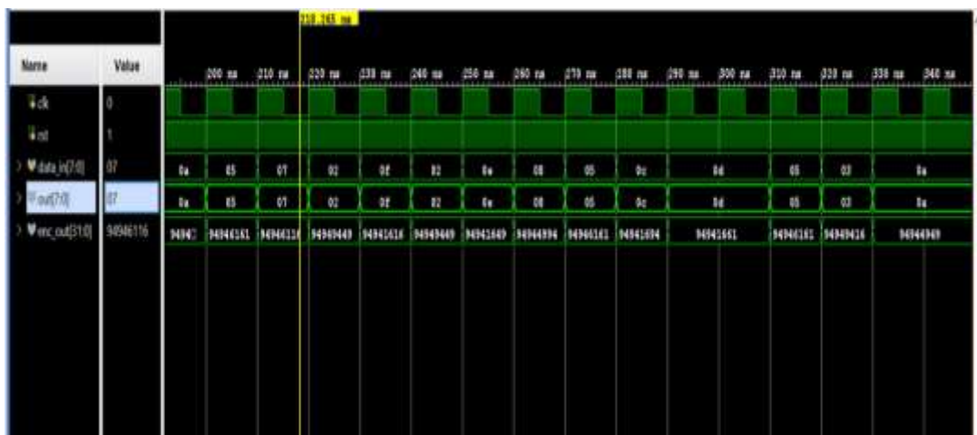
Figure 5. Simulation outcome
