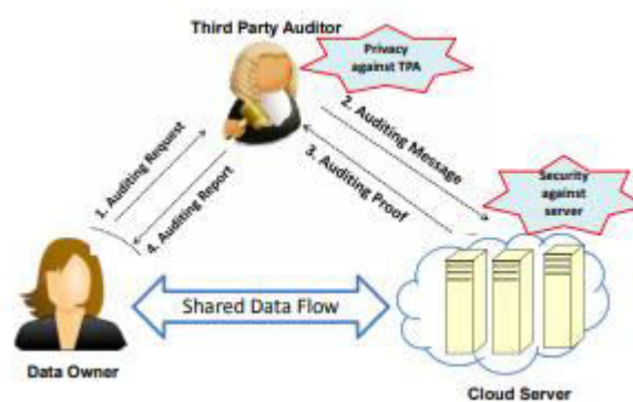
Figure 1. The system model of publicly verifiable remote data checking
