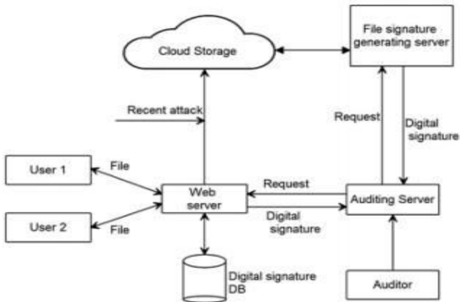
Figure 2. System Architecture
