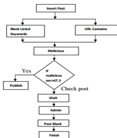
Fig. 3 Proposed Methodology
