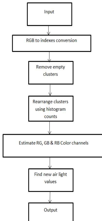
Fig 4. Process of estimate airlight
