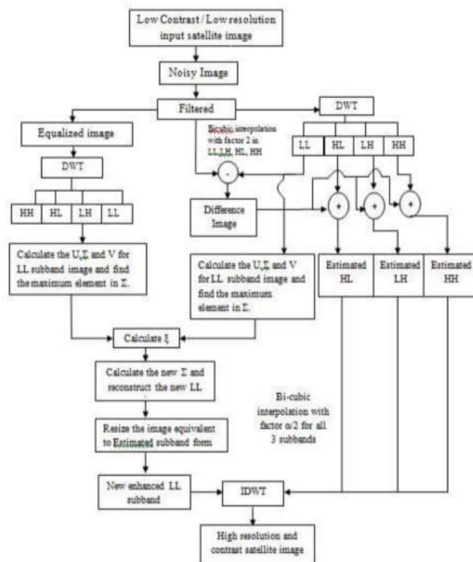
Fig 1: DE hazing using DWT
