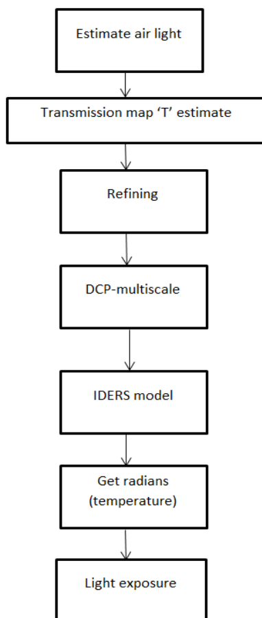
Fig 3. DE hazing using IDERS
