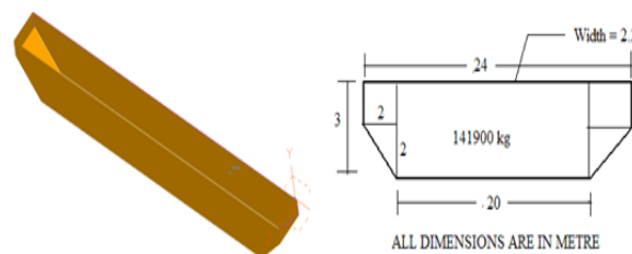
Figure 3. Solid model of Hopper in pro/e software
