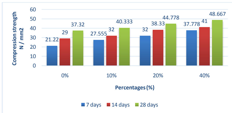
Figure 2. Graph representation of compression test (cubes)
