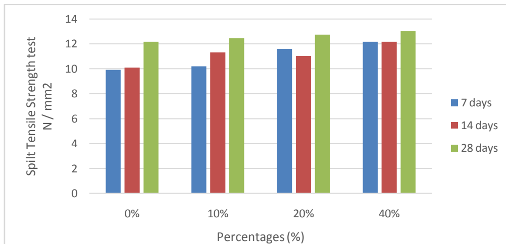
Figure 4. Graph representation of split tensile test
