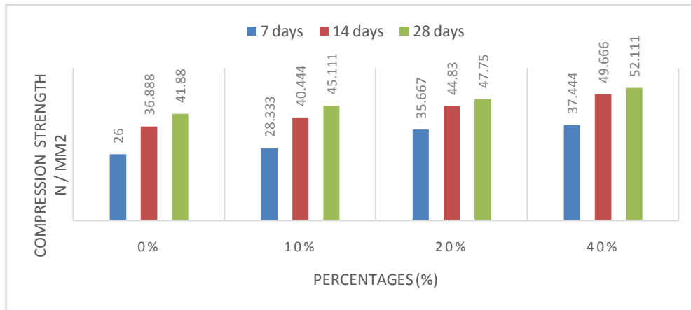
Figure 1. Graph representation of compression test (cubes)
