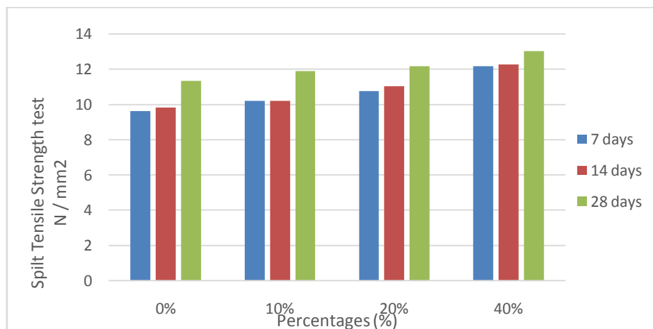
Figure 3. Graph representation of split tensile test (cylinders)
