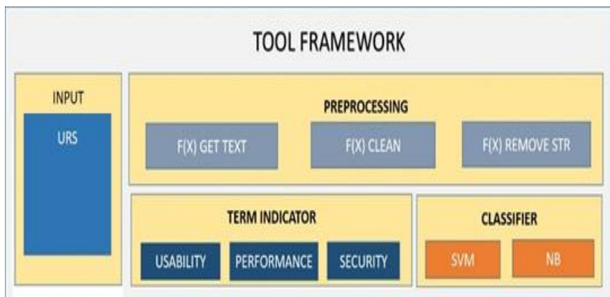
Figure 1.Tool Framework
