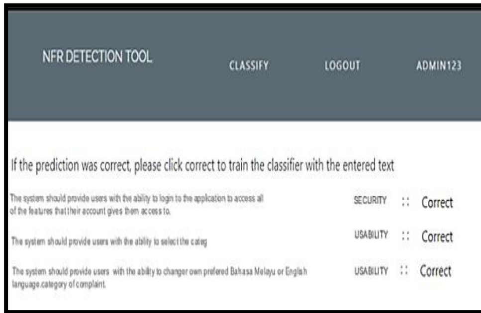
Figure 3. Classification Result
