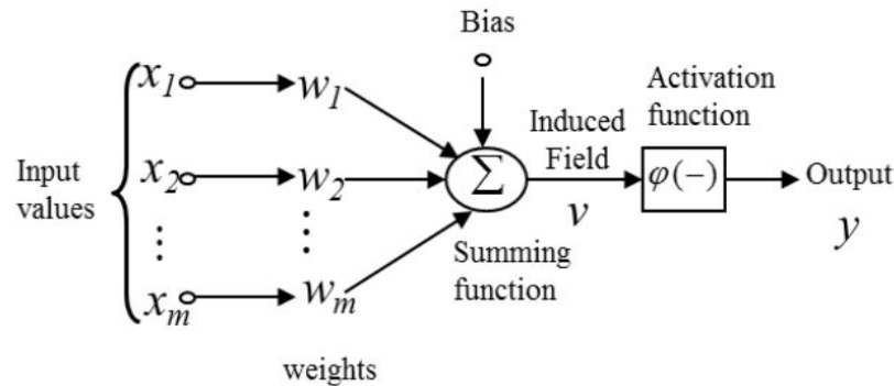
Fig. 2: Neuron diagram
