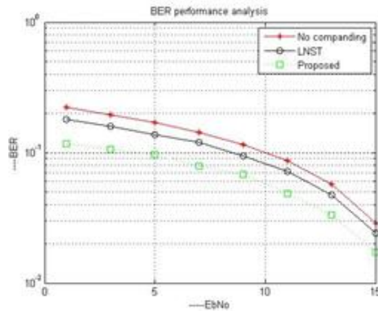
Fig.6 Performance analysis BER with AWGN
