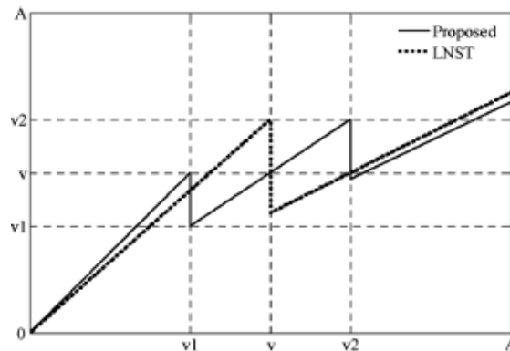
Fig.2 Profiles of companding transforms
