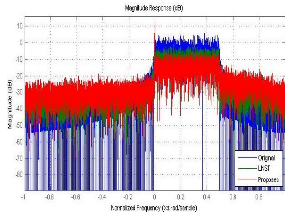
Fig.4 Power Spectrum magnitude response
