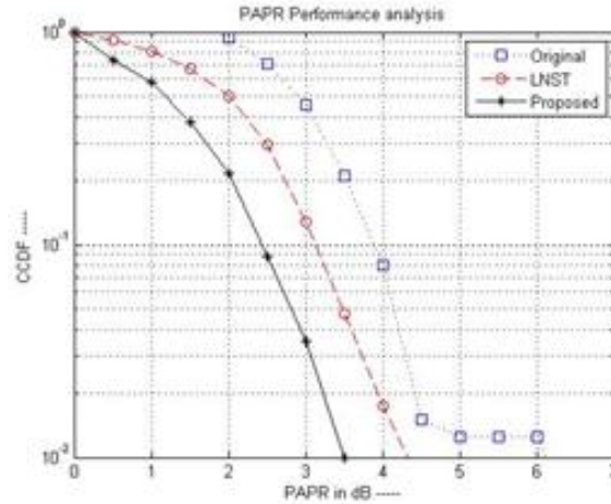
Fig.5 Performance analysis PAPR reduction
