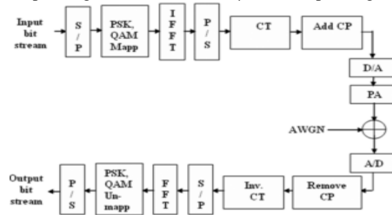
Fig.1 Block diagram of companded OFDM system
