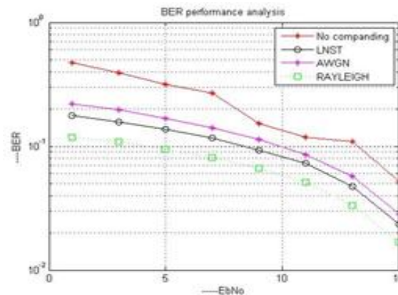
Fig.7 Performance analysis BER with AWGN and Rayleigh distribution
