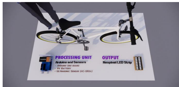
Figure.5. Top view
