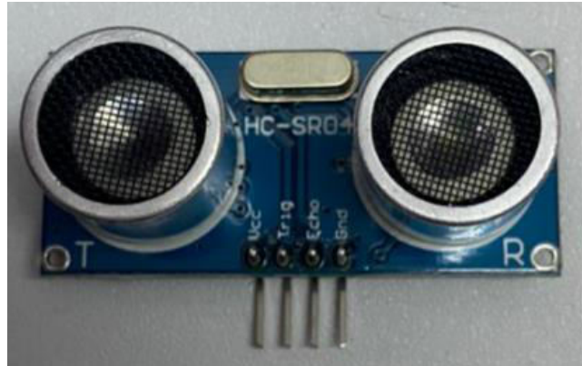
Figure.9. Ultrasonic distancing sensor
