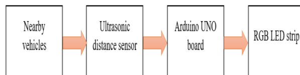
Figure.22. Block diagram
